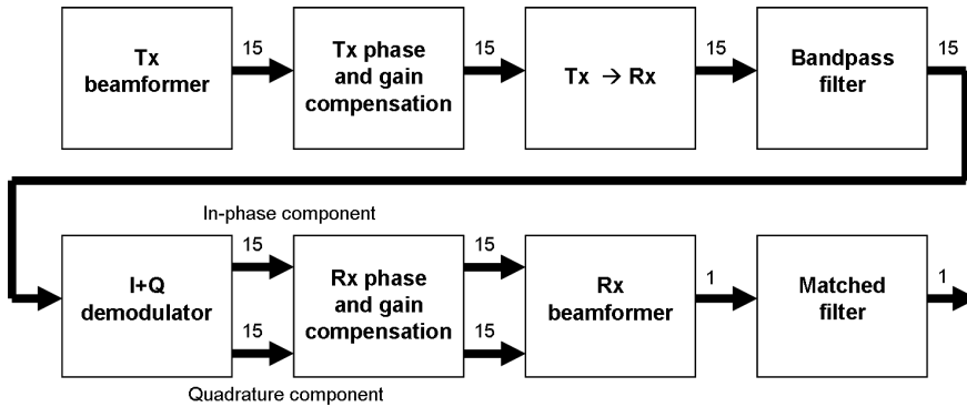
Fig. 2.2. Signal processing algorithm
