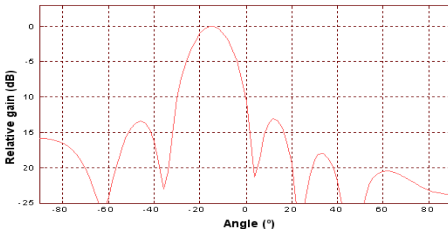
Fig. 5.4. Tx (-15)° beam pattern with 0° compensation
