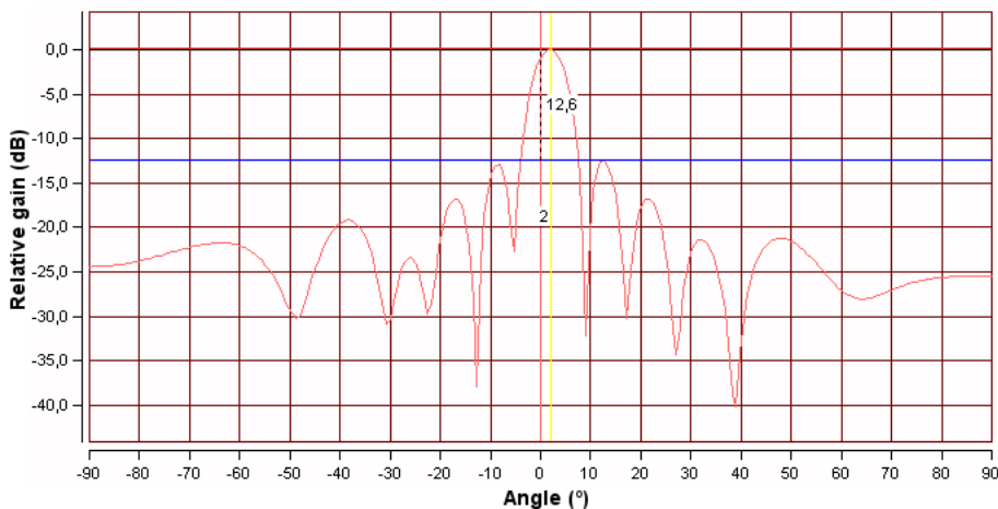
Fig. 4.3. Rx beampattern without compensation
