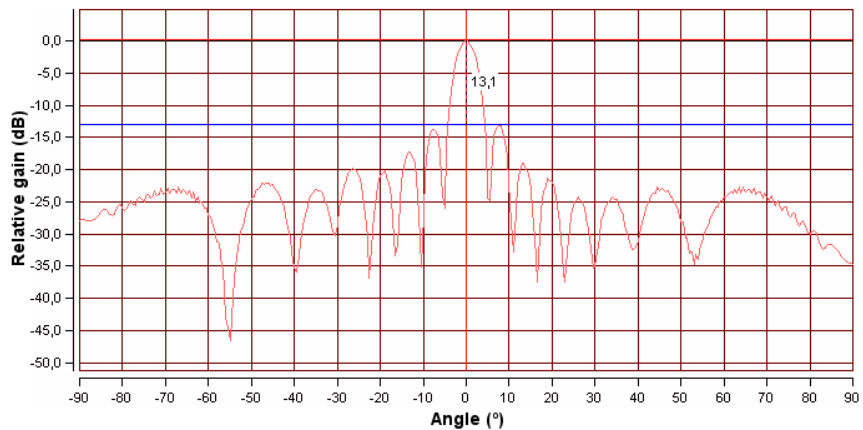
Fig. 3.5. Tx beampattern with compensation for 0°
