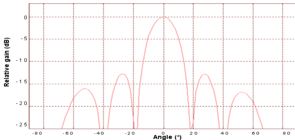
Fig. 5.3. Tx 0° beam pattern with compensation
