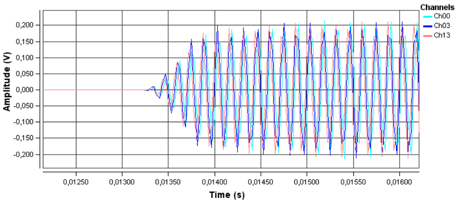
Fig. 3.1. Received signals from the Tx array
