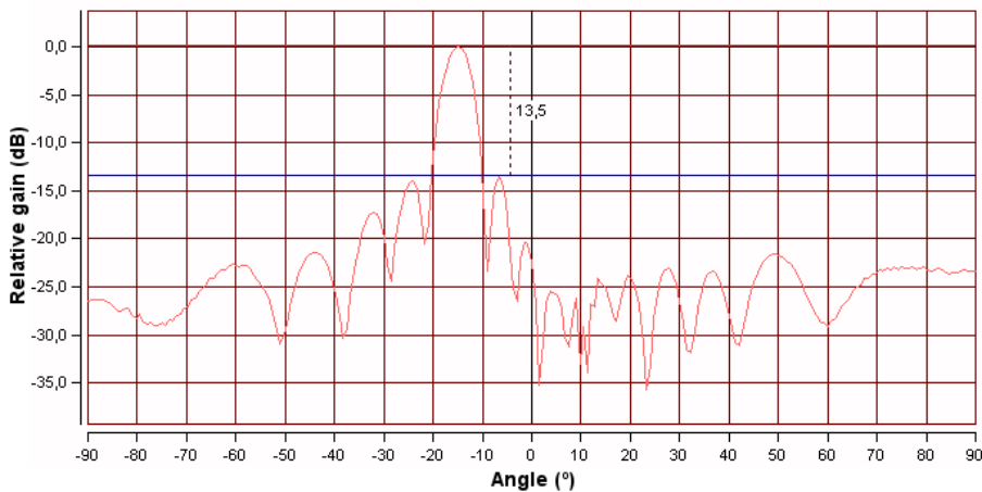
Fig. 3.6. Tx beampattern pointing to -15° with compensation for 0°
