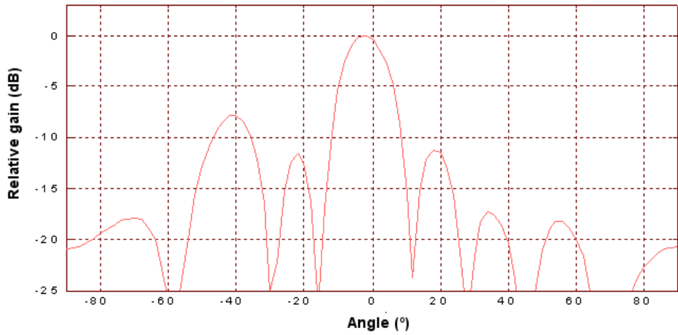
Fig. 5.5. Rx beampattern without compensation
