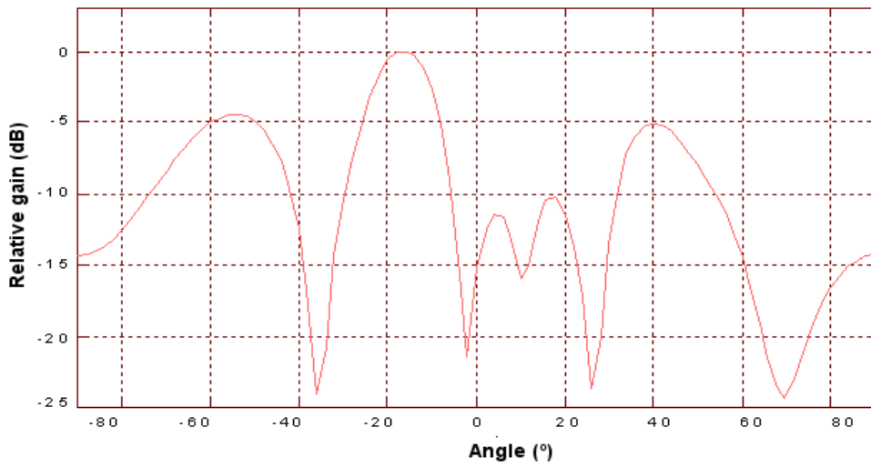
Fig. 5.7. Rx ( -15^\circ ) beampattern with compensation for 0^\circ
