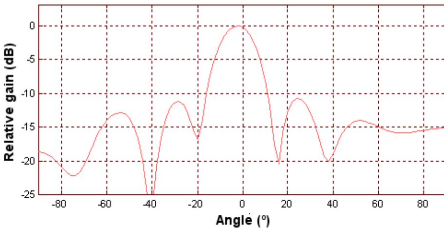
Fig. 5.2. Tx 0^\circ beampattern without compensation
