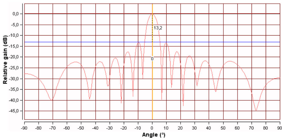
Fig. 4.4. Rx beampattern with compensation for 0°
